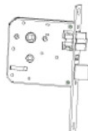
Deadbolt Mortise
