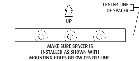
SPACER ORIENTATION
